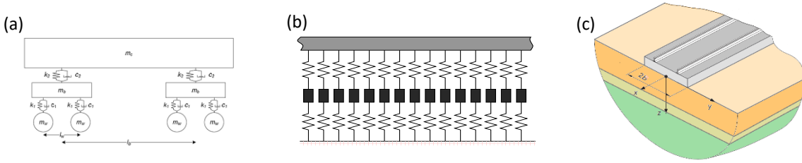
Fig. 1. (a) Vehicle model; (b) ballasted track model; (c) example of soil model.
